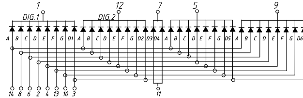
Common Cathode L-KLS9-D-3042 Ax
