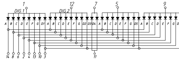
Common Anode L-KLS9-D-3042 Bx
